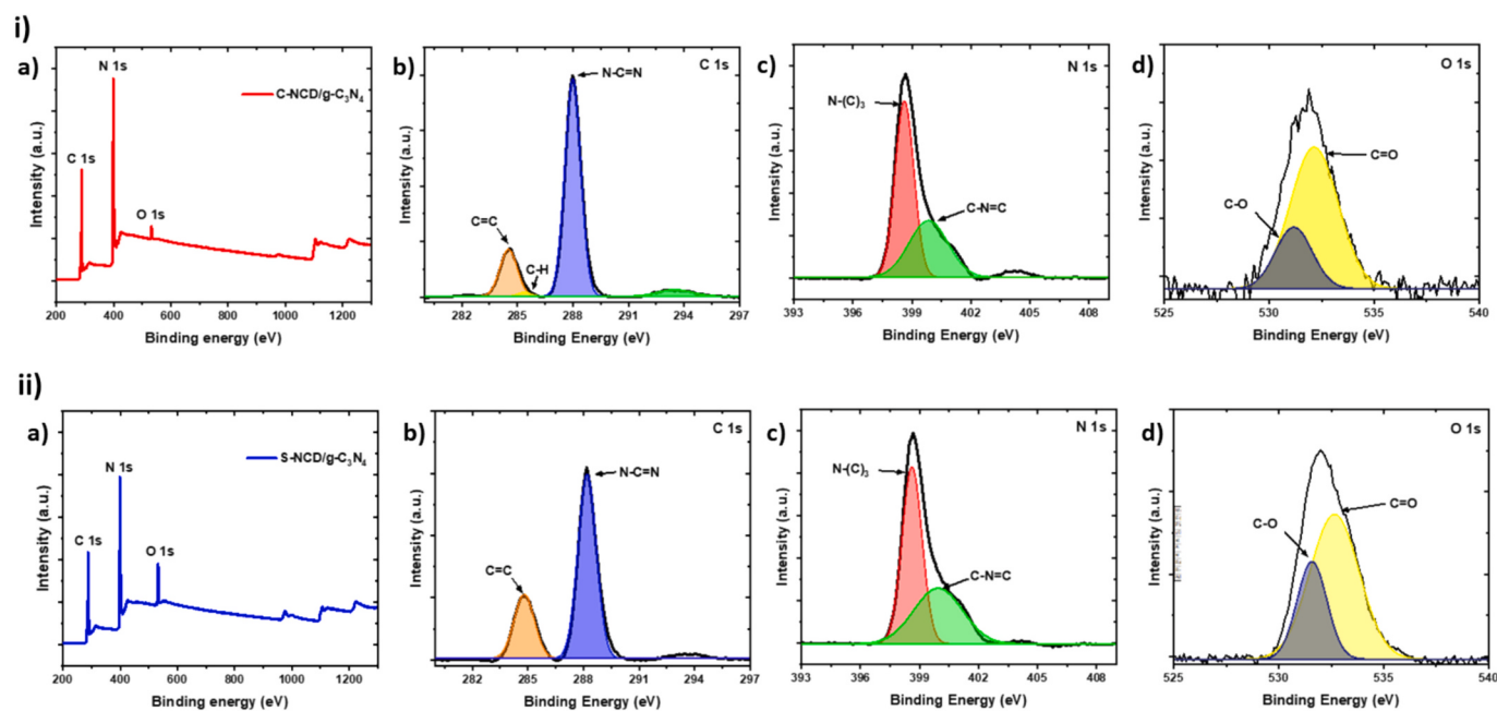
Fig. 3. XPS: i) C-NCD/g-C 3 N 4 and ii) S-NCD/g-C 3 N 4 .
