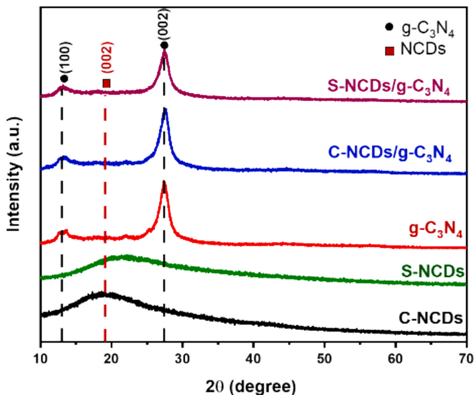
Fig. 1. XRD pattern of C-NCDs, S-NCDs, g-C 3 N 4 , C-NCDs/ g-C 3 N 4 , and S-NCDs/ g-C 3 N 4 .
