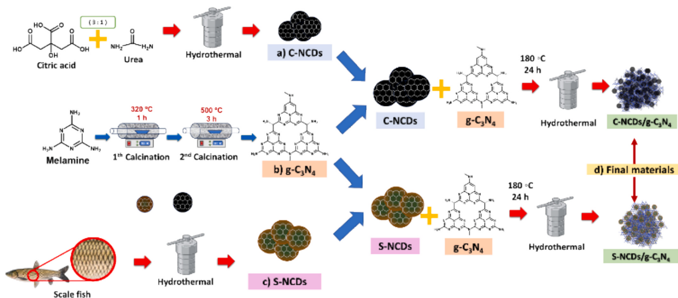
Scheme 1. Synthesis: a) C-NCDs, b) g- \text{C}_3\text{N}_4 , c) S-NCDs, and d) NCDs/g- \text{C}_3\text{N}_4 .
