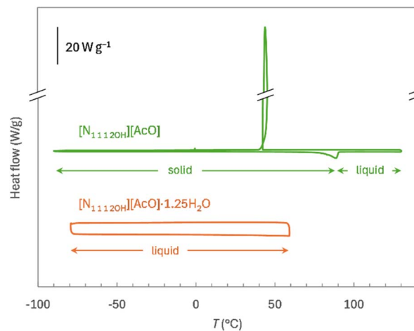
Fig. 1 Second cycle thermographs of [N 1.1.1.2 OH][AcO] (green) and [N 1.1.1.2 OH][AcO]·1.25H 2 O (orange) measured by DSC (offset along the y axis for clarity), showing the solid and liquid ranges for the former, delimited by the melting point (down peak at 88 °C), and the fully liquid range for the latter. Up-signals indicate exothermic events; heating/cooling rates: 5 °C min -1 ; carrier gas: N 2 (50 mL min -1 ).
