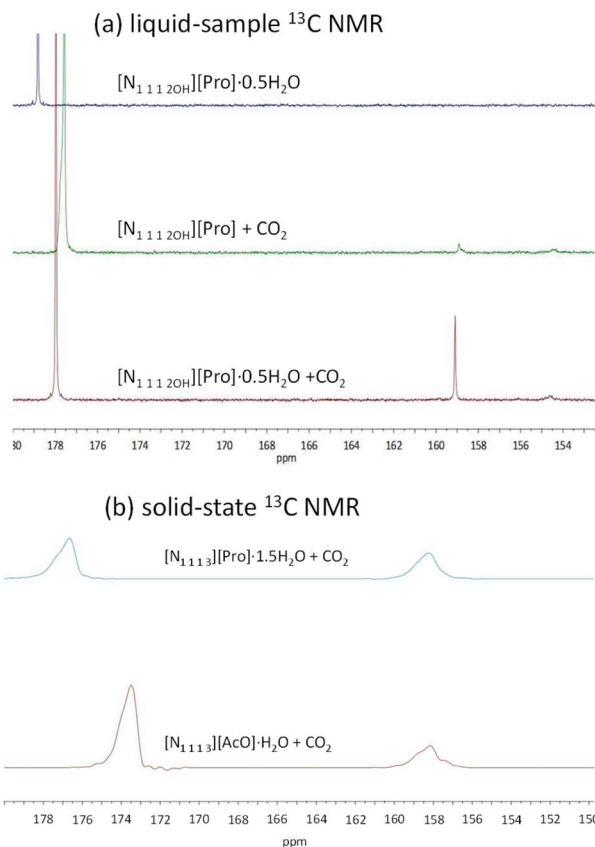
Fig. 5 (a) Liquid-sample ^{13}\text{C} NMR spectra of [\text{N}_{1112}\text{OH}][\text{Pro}]\cdot 0.5\text{H}_2\text{O} , \text{CO}_2 -saturated [\text{N}_{1112}\text{OH}][\text{Pro}] , and \text{CO}_2 -saturated [\text{N}_{1112}\text{OH}][\text{Pro}]\cdot 0.5\text{H}_2\text{O} , using \text{DMSO}-d_6 in a sealed capillary tube as an external standard. (b) Solid-state magic-angle spinning (MAS) ^{13}\text{C} NMR spectra of \text{CO}_2 -saturated [\text{N}_{1113}][\text{Pro}]\cdot 1.5\text{H}_2\text{O} , and \text{CO}_2 -saturated [\text{N}_{1113}][\text{AcO}]\cdot \text{H}_2\text{O} .
