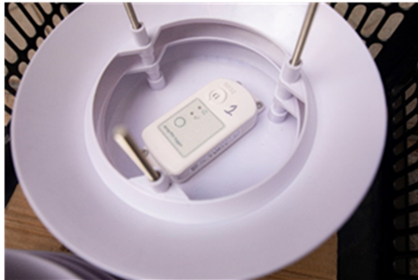
Figure 3. Meteorological sensor integrated into the screen protector. Source: Òscar Saladié.
