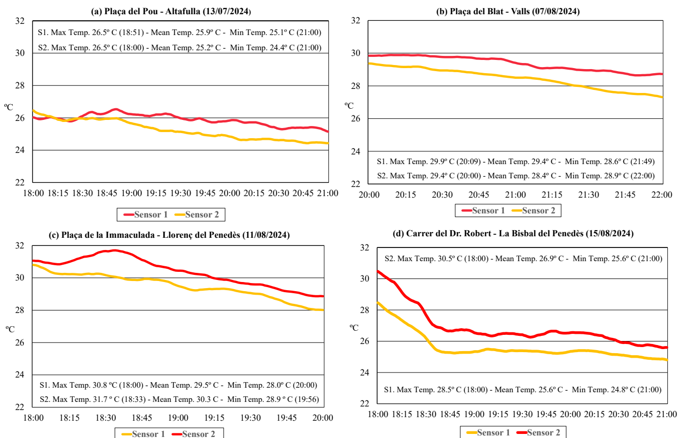
Figure 8. Temperature evolution during human tower exhibitions.
