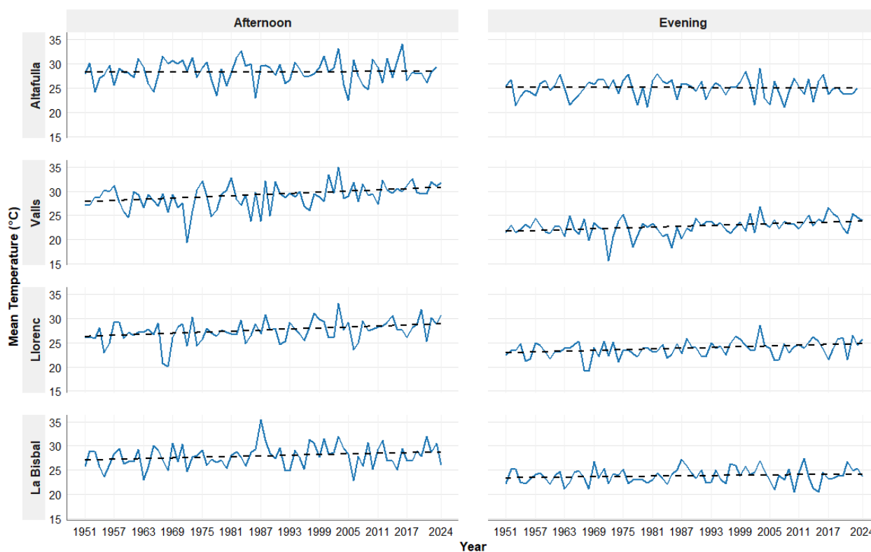
Figure 5. Mean temperature from 12:00 to 15:00 ( left ) and from 18:00 to 21:00 (from 20:00 to 22:00 in the case of Valls) ( right ) on the 2nd Saturday of July in Altafulla; 1st Wednesday of August in Valls; 2nd Sunday of August in Llorenç del Penedès; and 15 August in La Bisbal del Penedès (1951–2024). Dash line shows the trend.
