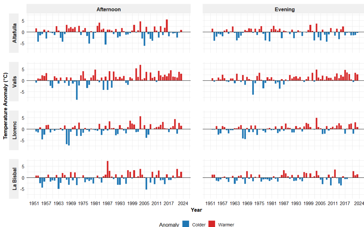
Figure 6. Temperature anomalies from 12:00 to 15:00 (left) and from 18:00 to 21:00 (right) on the 2nd Saturday of July in Altafulla; 1st Wednesday of August in Valls; 2nd Sunday of August in Llorenç del Penedès; and 15 August in La Bisbal del Penedès (1951–2024).
