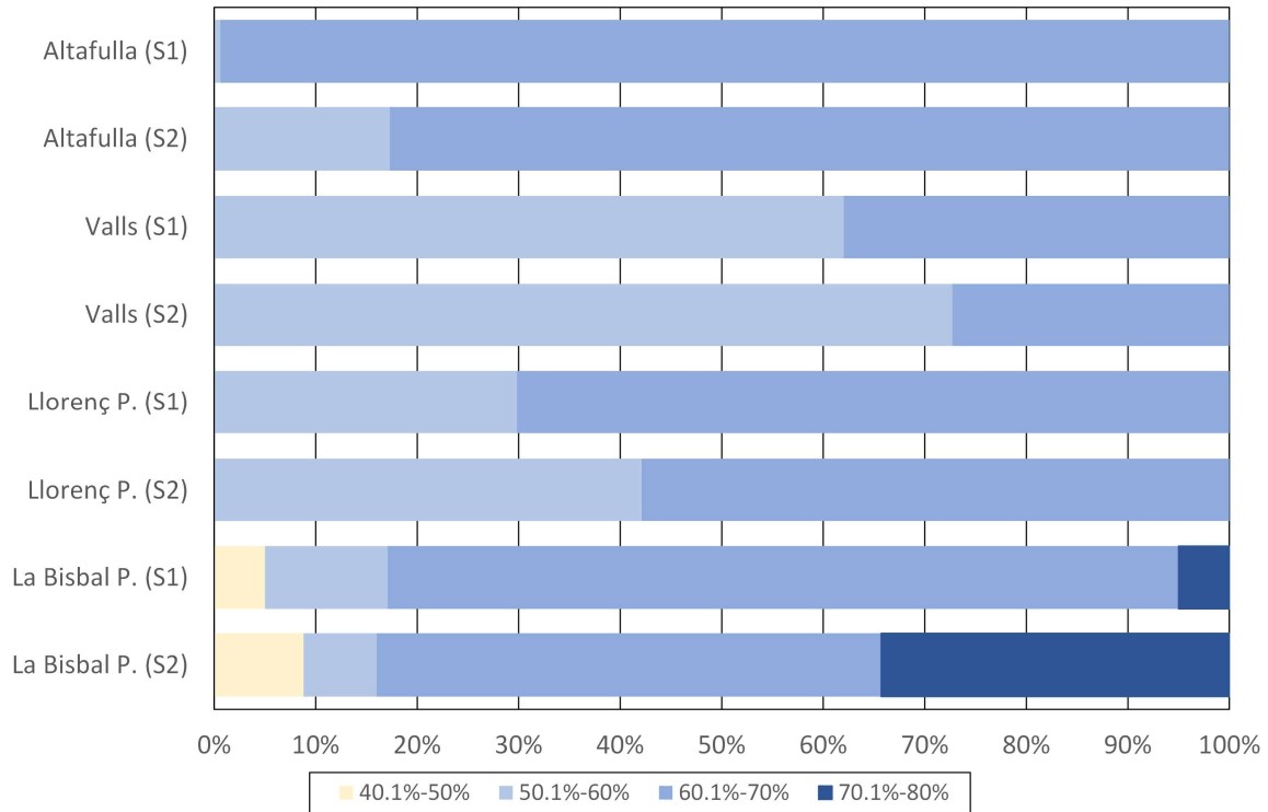
Figure 9. Distribution of the duration of human tower exhibitions according to relative humidity.
