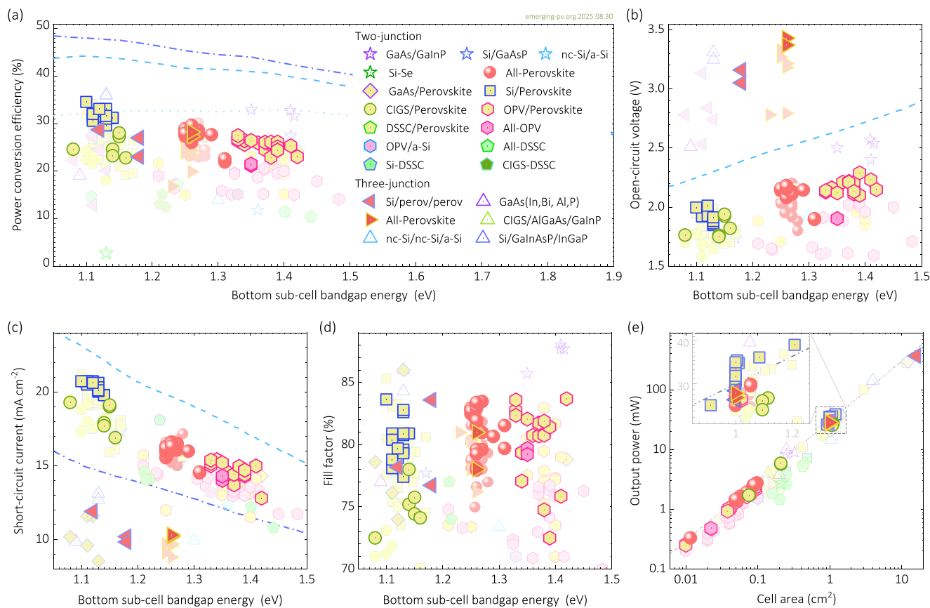
FIGURE 4 | Highest-PCE values for monolithic (two-terminal) multijunction photovoltaic research cells with up to three junctions. Performance parameters are shown as a function of the absorber bandgap energy of the bottom sub-cell for different photovoltaic technologies: (a) PCE, (b) open-circuit voltage, (c) short-circuit current density, and (d) fill factor, along with (e) output power versus device area. The dotted, dashed, and dash-dotted lines in (a-c) represent the detailed balance efficiency limits for single-junction, double-junction (optimized top sub-cell), and triple-junction (optimized top and middle sub-cells) devices, respectively [37, 31]. In (e), the dash-dot-dot line corresponds to the efficiency isoline for PCE = 30% and the inset magnifies the \sim 1 cm 2 -area results. Data points are represented by light-colored symbols for reports published before August 2024 and by opaque symbols for those published thereafter.
